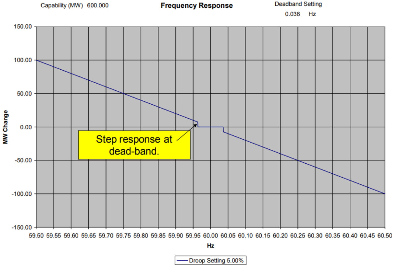
Figure 4.2: Governor Deadband Setting with Step Implementation 13
