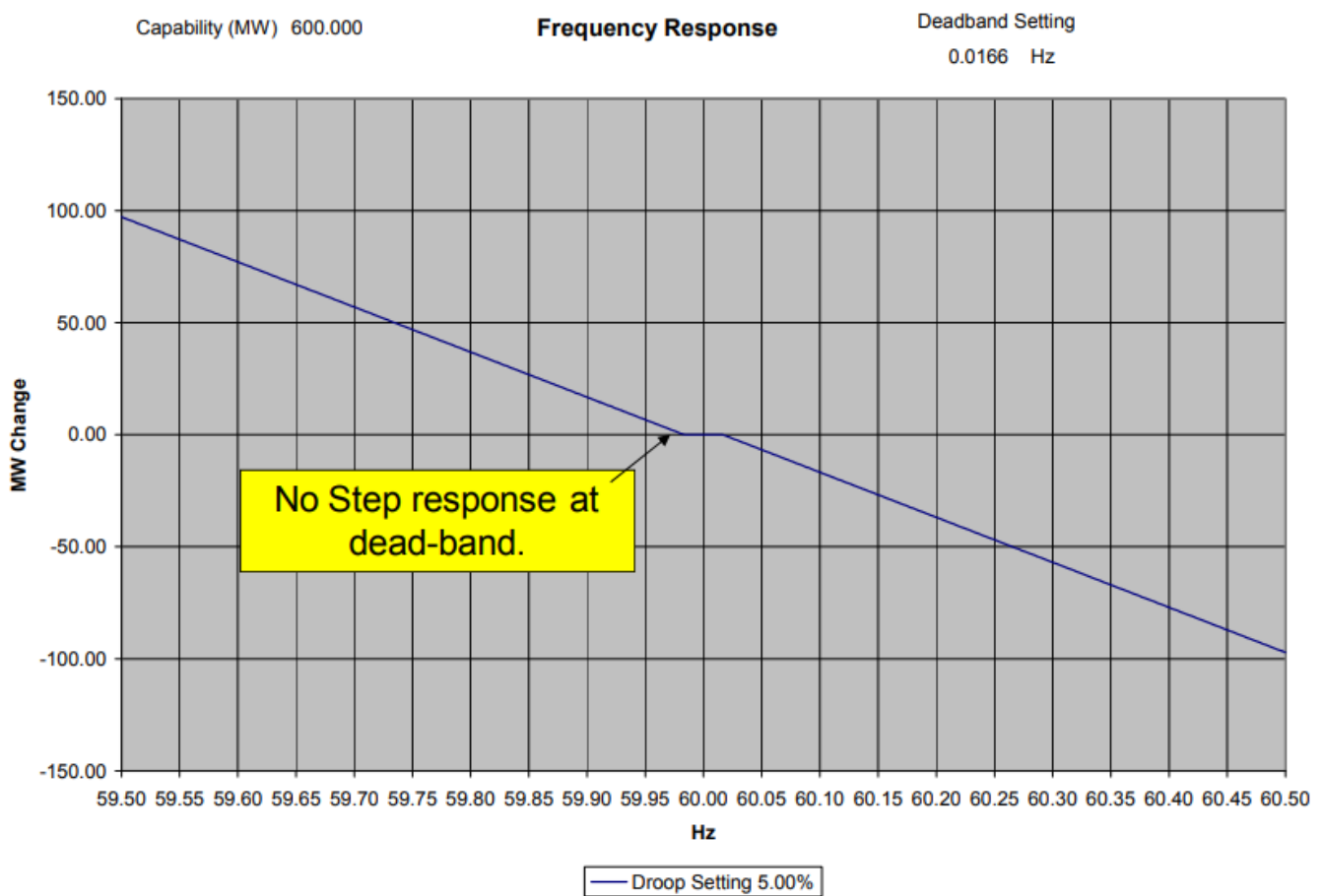
Figure 4.1: Governor Deadband Setting without Step Implementation 1112
