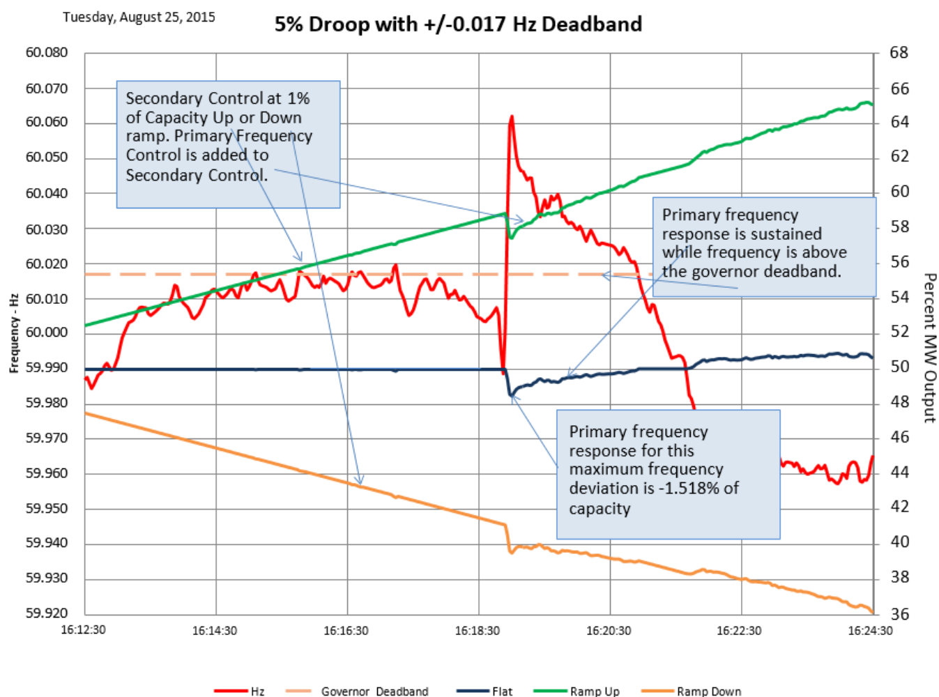
Figure 3.4: Example of Properly Coordinated Primary Frequency Control while Ramping MW Up or Down Via Local or Remote Control or while Operating at a Fixed MW Output in the Graph Above - High Frequency Excursion with a Lower Deadband (Deadband = 17 mHz)
