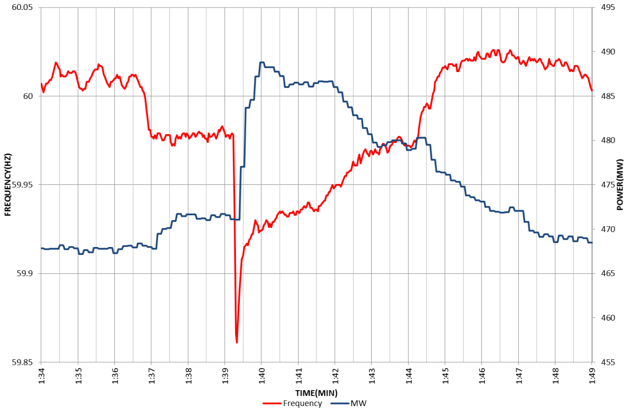
Figure A.1: Combined-Cycle Unit/Block Responding to Low Frequency Event at 17 mHz Deadband
