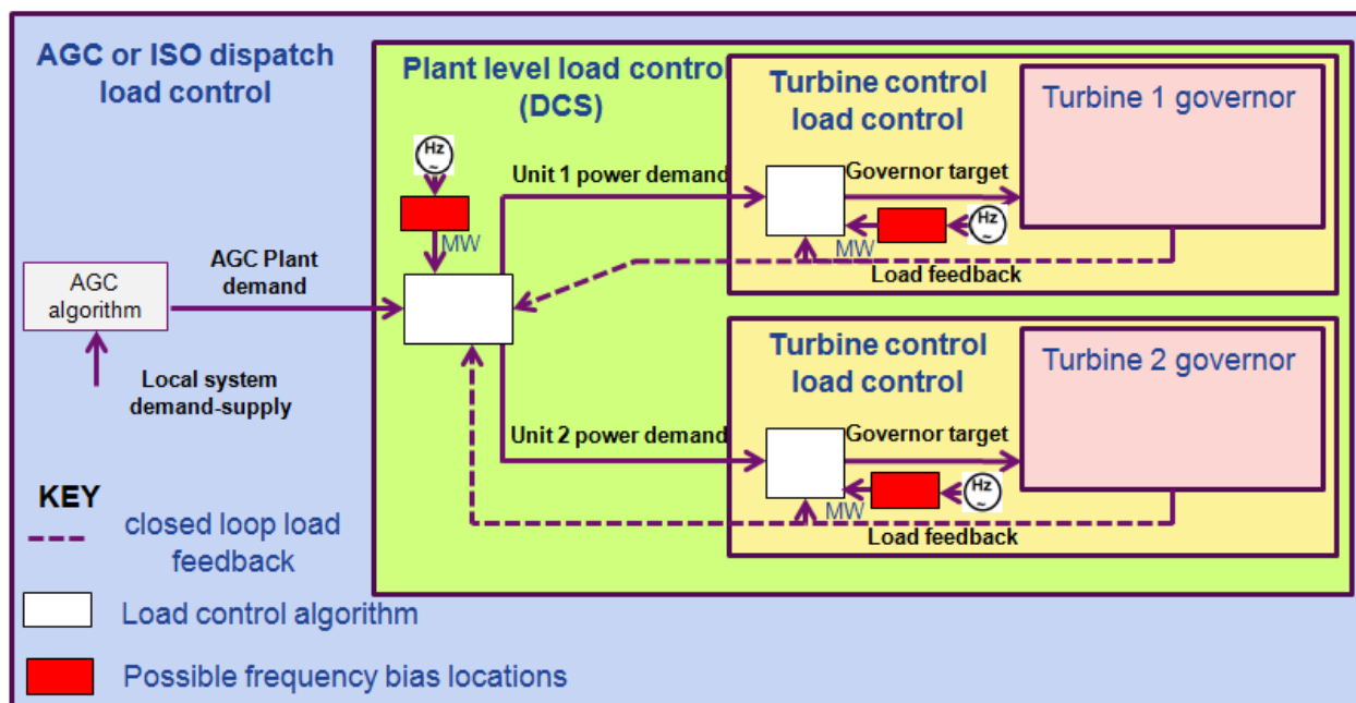
Figure 3.2: Typical High Level Generating Resource Control System
