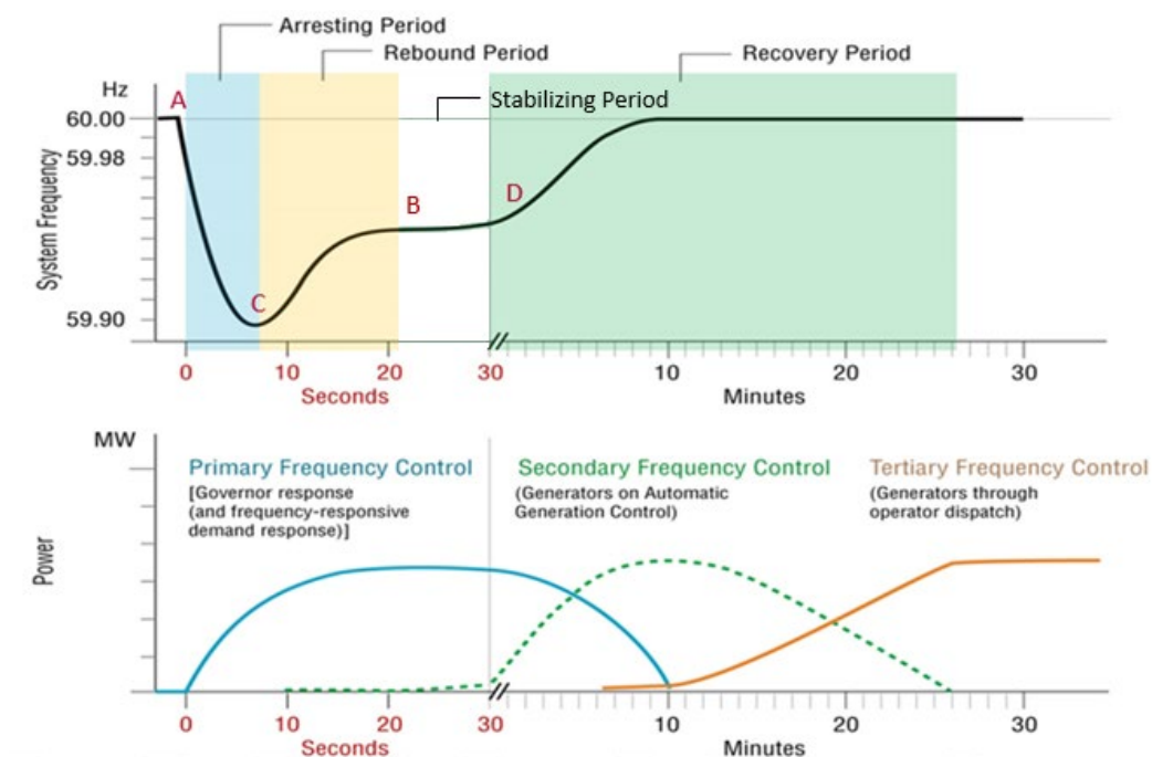
Figure 2.1: The Sequential Actions and Impacts on System Frequency of Primary, Secondary, and Tertiary Frequency Control 1
