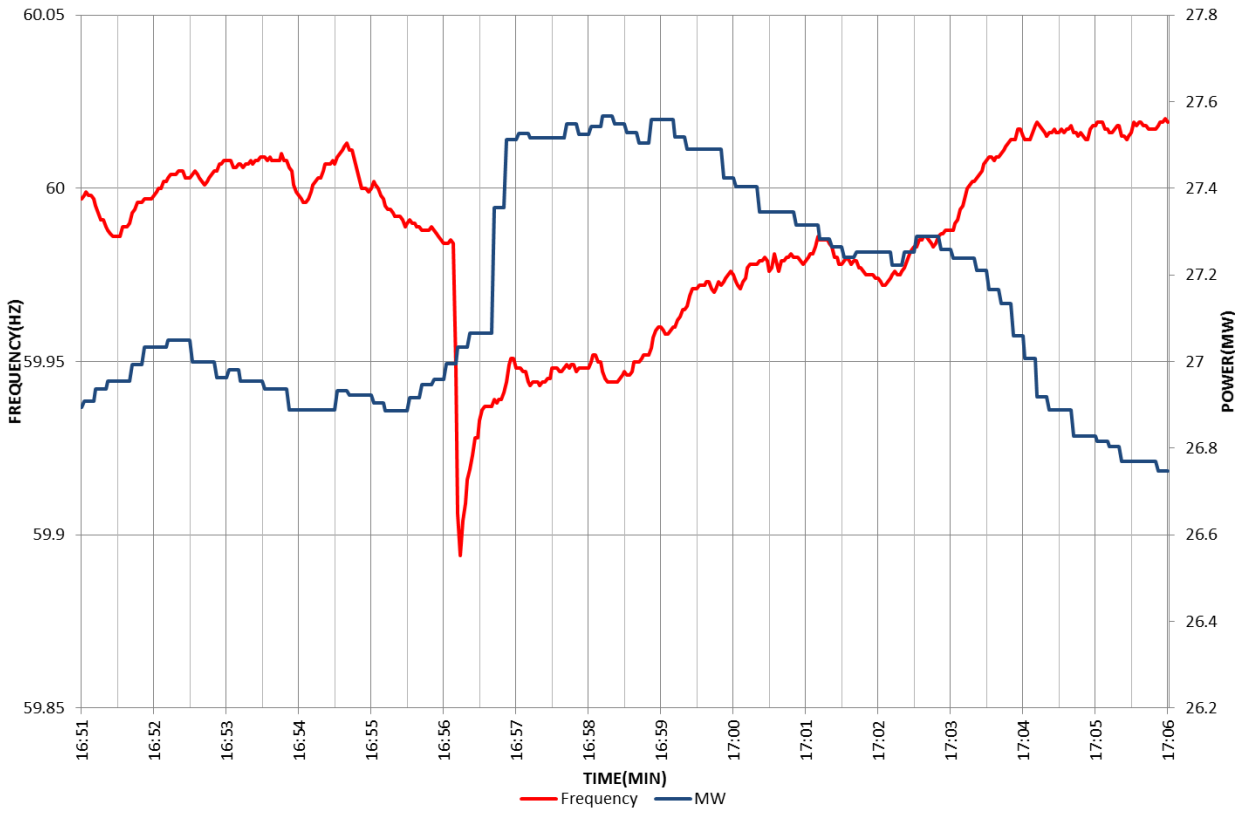
Figure A.6: Hydro Resource Responding to Low Frequency Event at 17 mHz Deadband and Five Percent Droop
