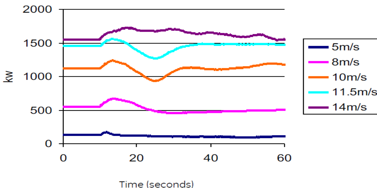
Figure 3.6: Fast Frequency Control Response of Wind Turbine at Different Wind Speed Conditions
