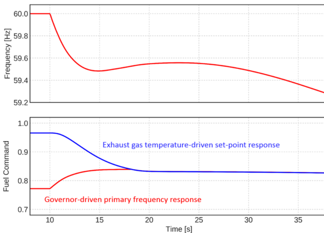
Figure 3.5: Exhaust Gas Temperature Controls on Gas Turbines Will Decrease Primary Frequency Response if Frequency Remains Depressed 5
