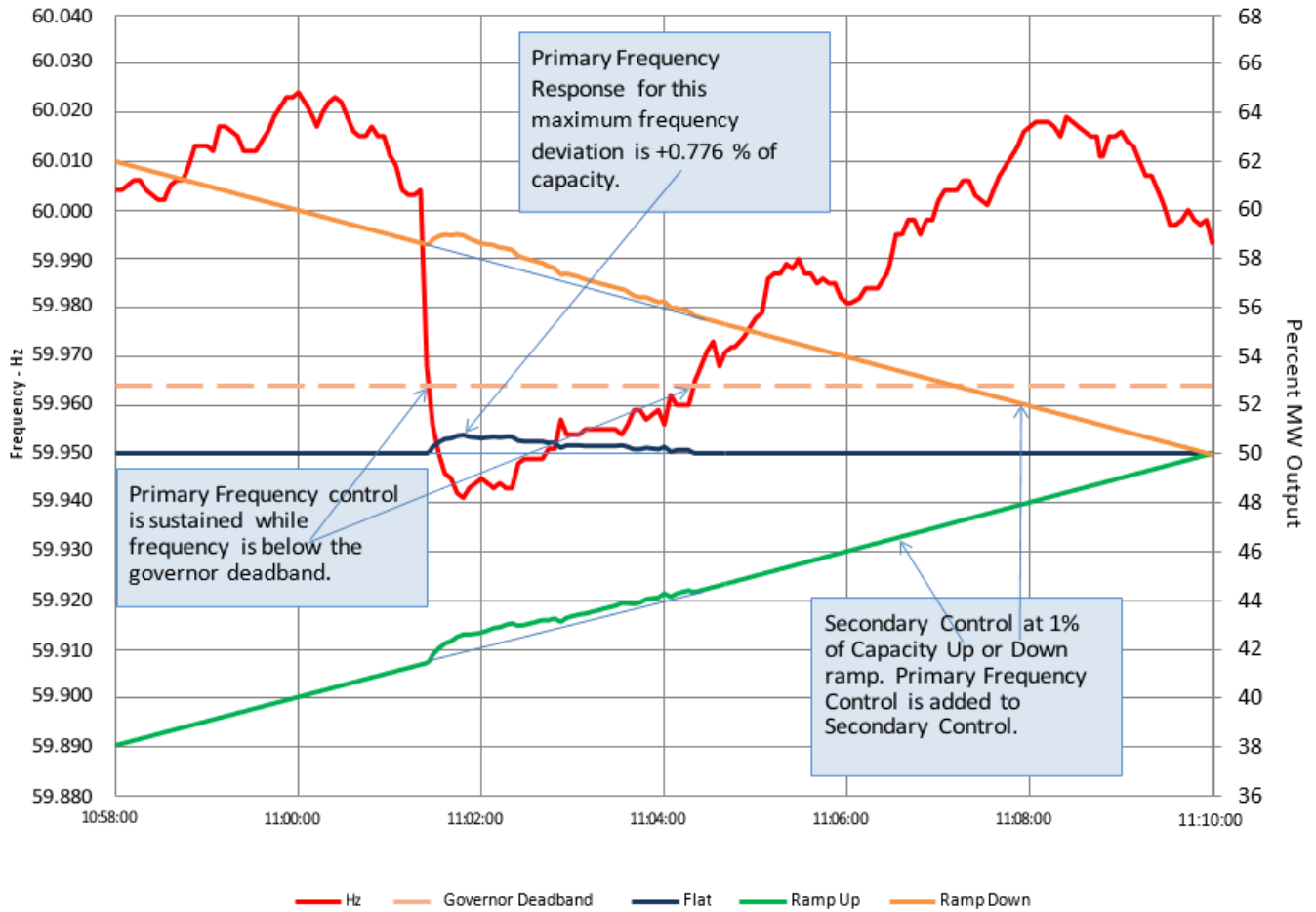
Figure 3.3: Example of Properly Coordinated Primary Frequency Control while Ramping MW Up or Down via Local or Remote Control or While Operating at a Fixed MW Output (Deadband)
