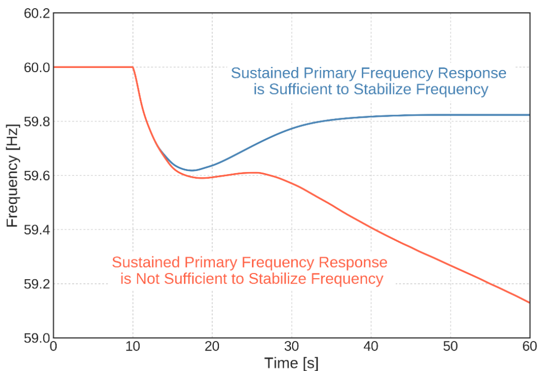
Figure 3.1: Sustaining vs Nonsustaining Primary Frequency Response Effect on System Frequency 4
